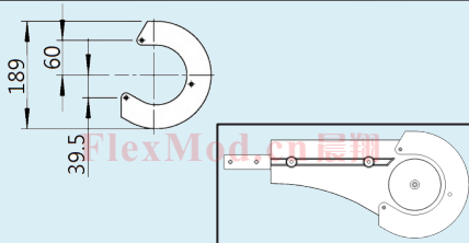
CXMSJ 189 Protective cover for idler end unit (尾端防护罩)
