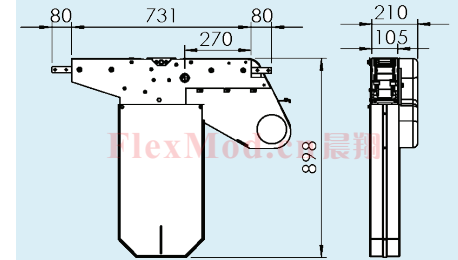
CXKEC 0HL Drive unit (驱动单元) Transmission on left-hand side (传动装置在左侧)
