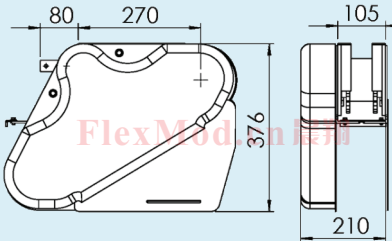
CXKEB 0HRA Drive unit (驱动单元) Transmission on right-hand side (传动装置在右侧)
