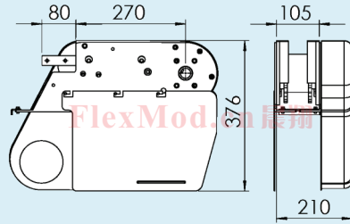
CXKEB 0HLA Drive unit (驱动单元) Transmission on left-hand side (传动装置在左侧)
