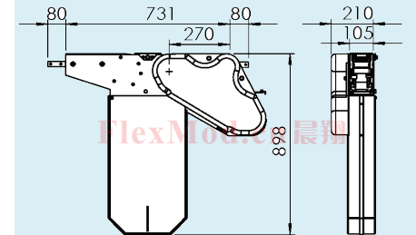
CXKEC 0HR Drive unit (驱动单元) Transmission on right-hand side (传动装置在右侧)
